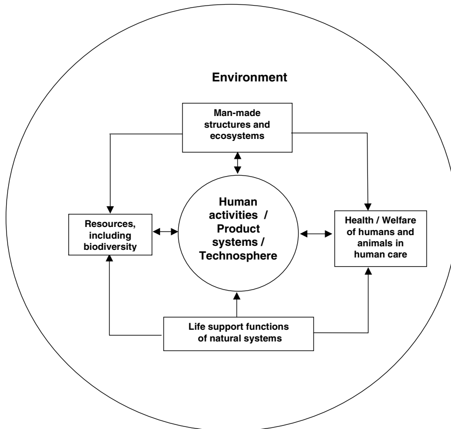
Fig. 1: Areas of protection and their relations
