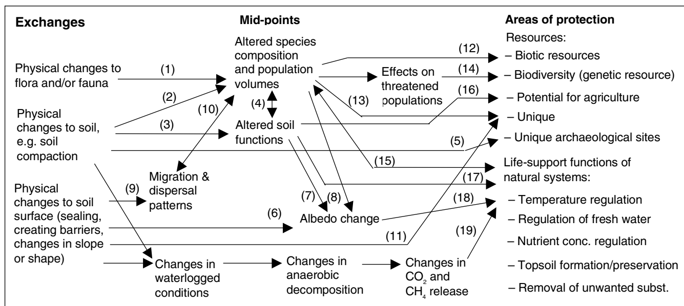
Fig. 2: Impact chains for physical impacts of land use
