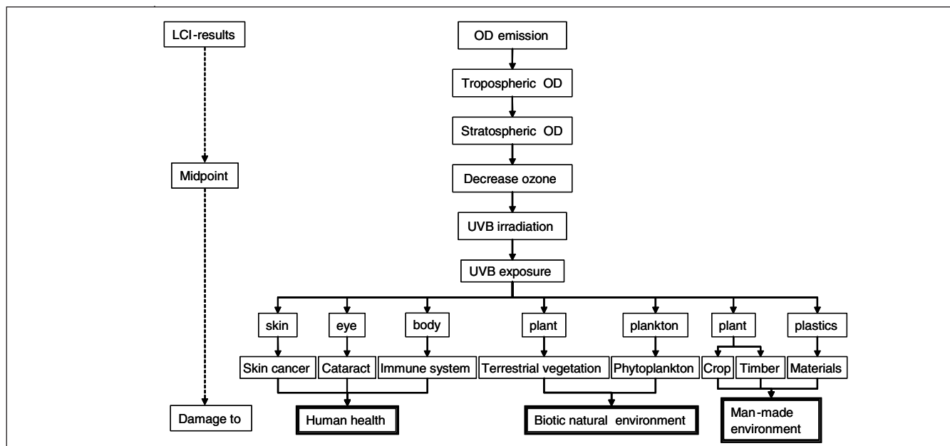
Fig. 2: Example of a pathway structure linking ozone depleting emissions to impacts on human health, biotic natural environment and man-made environment (adapted from Itsubo et al. 2004)
